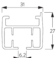
SG 10925 Profile
